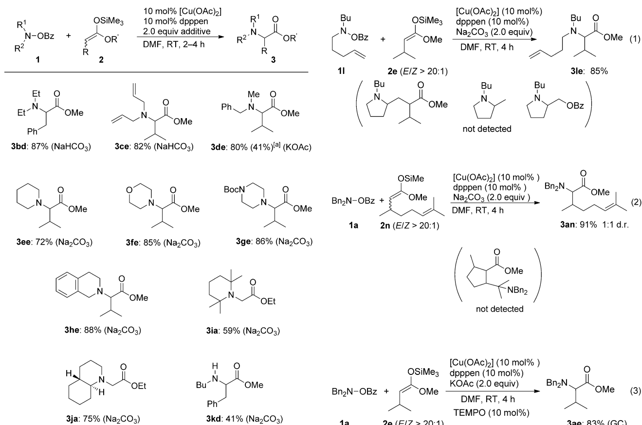
Scheme 1. Copper-catalyzed electrophilic amination of the ketene silyl acetals 2 with various hydroxylamines ( 1 ) using the reaction conditions detailed in Table 2. [a] Used 1.2 equiv of 2 and \text{KOAc} . The additive is given in parentheses. Boc = tert -butoxycarbonyl.
